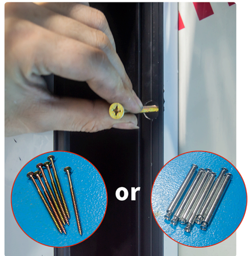
c. Fixed installation screw
